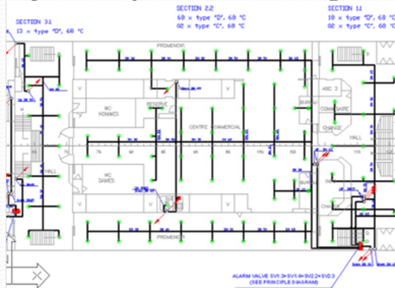
Sprinkler System One Line Diagrams
